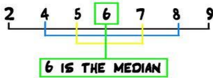
Graph 3.8: Example of Median
