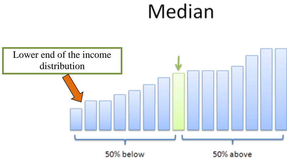
Graph 3.9: Example of Median
